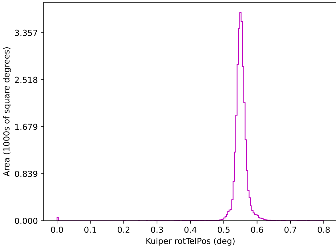
ddf_loaded_half_f14_v3.4_10yrs z: Kuiper rotTelPos
