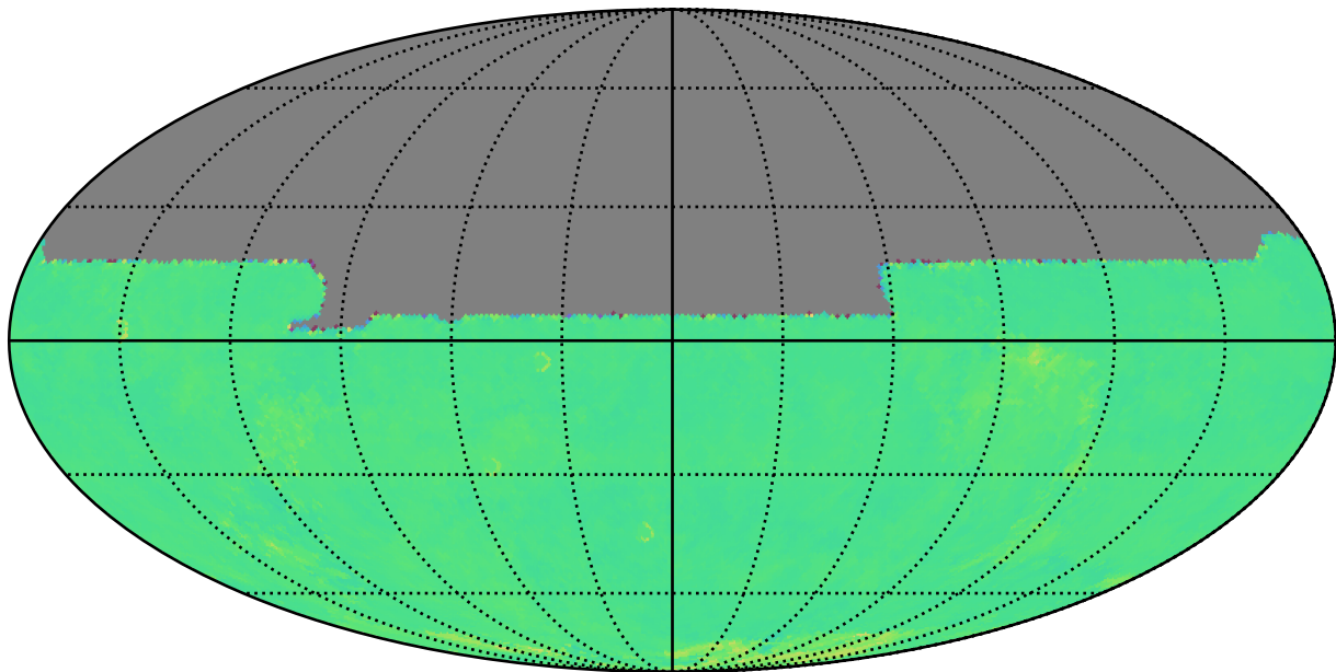
ddf_loaded_half_fl4_v3.4_10yrs y: Kuiper rotTelPos
