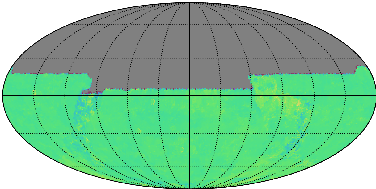
ddf_loaded_half_fl4_v3.4_10yrs u: Kuiper rotTelPos
