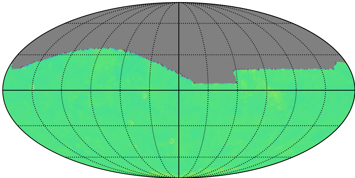
ddf_loaded_half_fl4_v3.4_10yrs r: Kuiper rotTelPos
