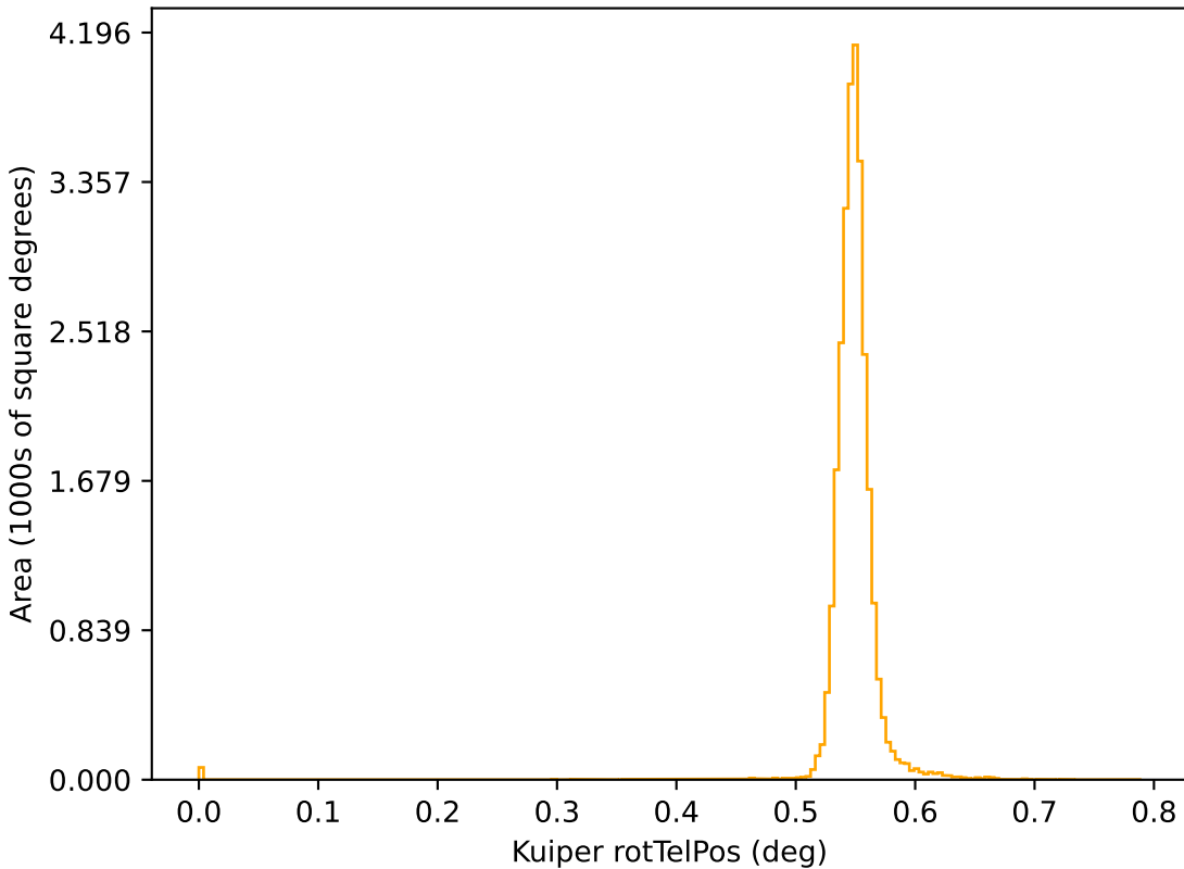
ddf_loaded_half_fl4_v3.4_10yrs r: Kuiper rotTelPos
