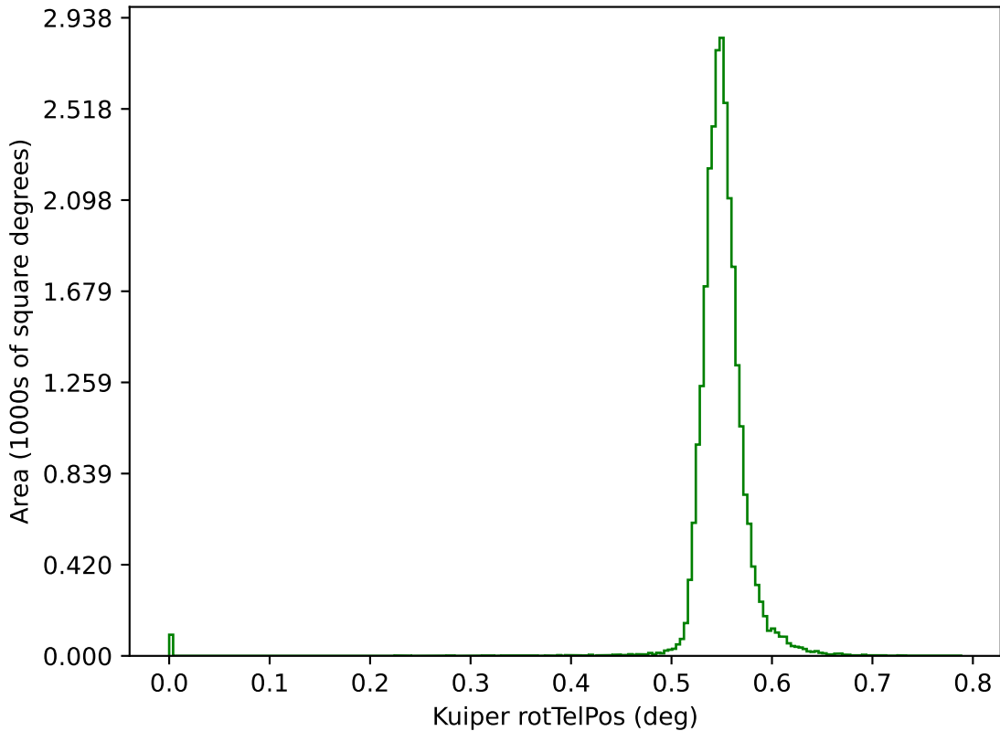
ddf_loaded_half_fl4_v3.4_10yrs g: Kuiper rotTelPos
