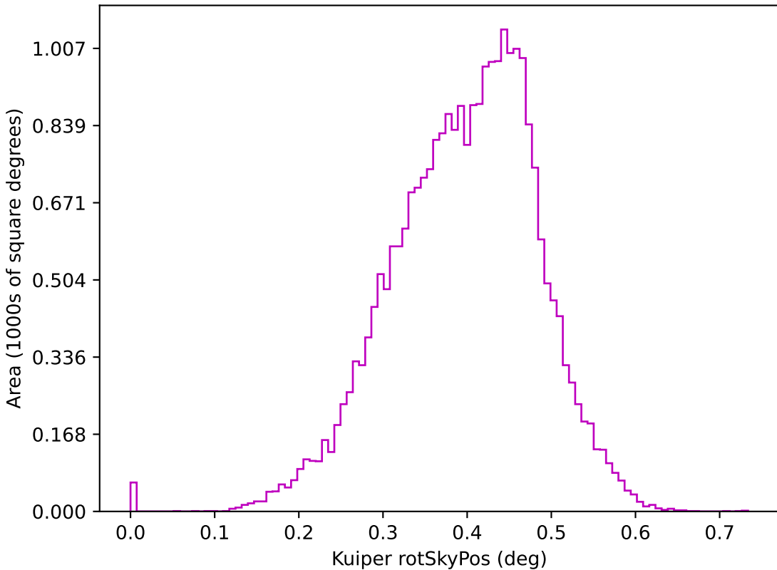
ddf_loaded_half_fl4_v3.4_10yrs z: Kuiper rotSkyPos
