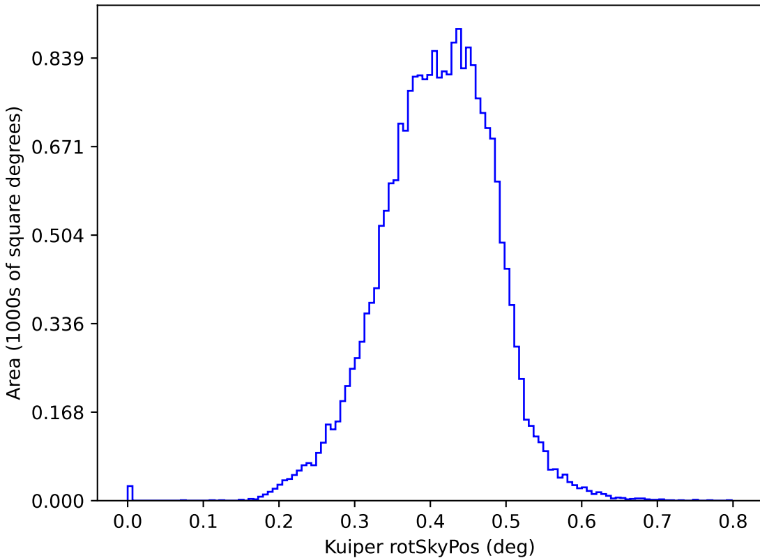
ddf_loaded_half_fl4_v3.4_10yrs y: Kuiper rotSkyPos
