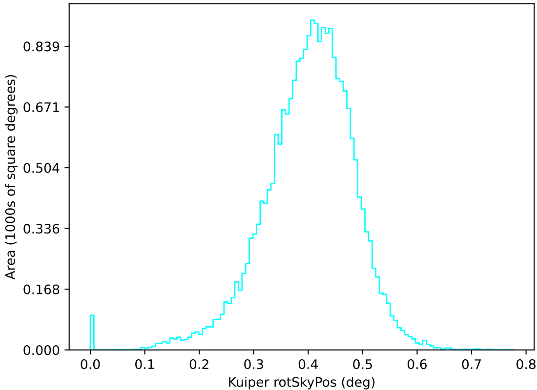
ddf_loaded_half_fl4_v3.4_10yrs u: Kuiper rotSkyPos
