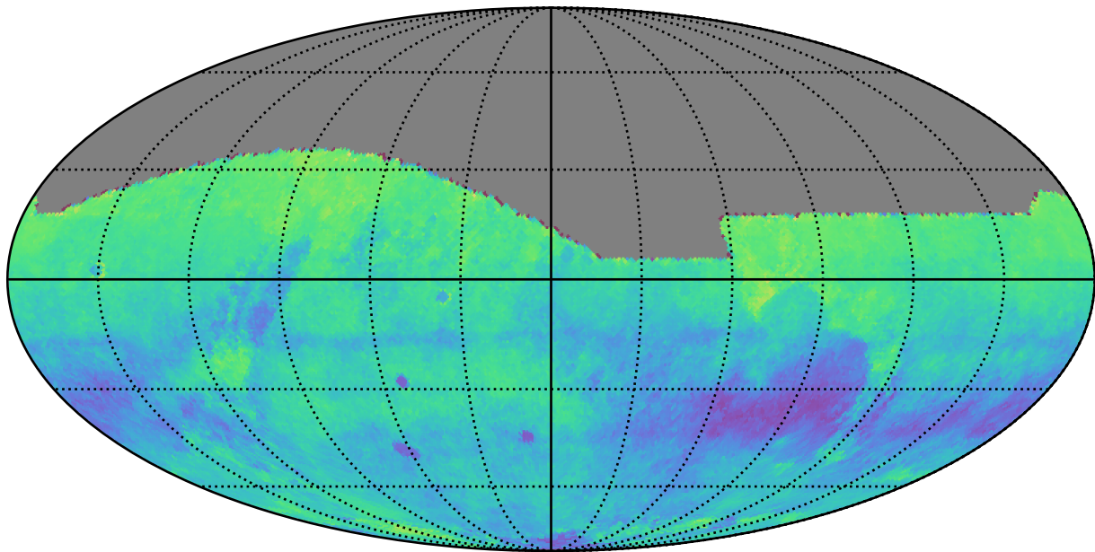
ddf_loaded_half_fl4_v3.4_10yrs r: Kuiper rotSkyPos
