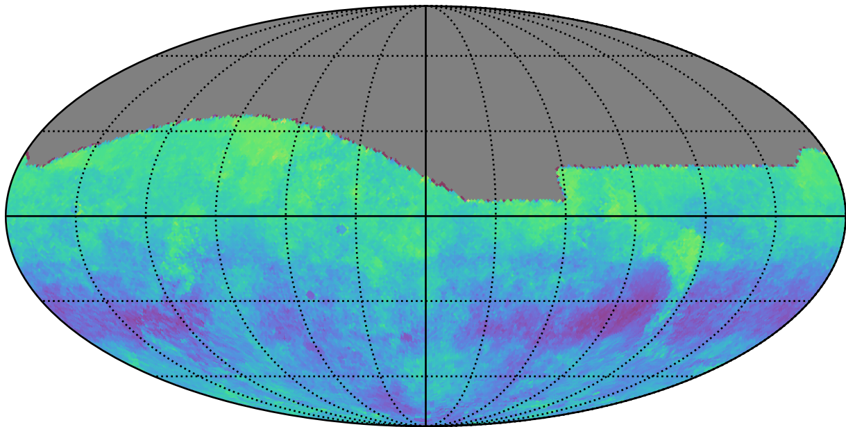
ddf_loaded_half_fl4_v3.4_10yrs g: Kuiper rotSkyPos
