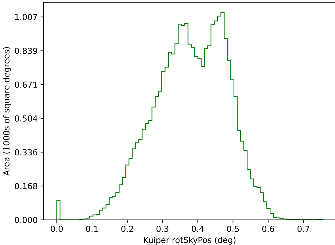
ddf_loaded_half_fl4_v3.4_10yrs g: Kuiper rotSkyPos
