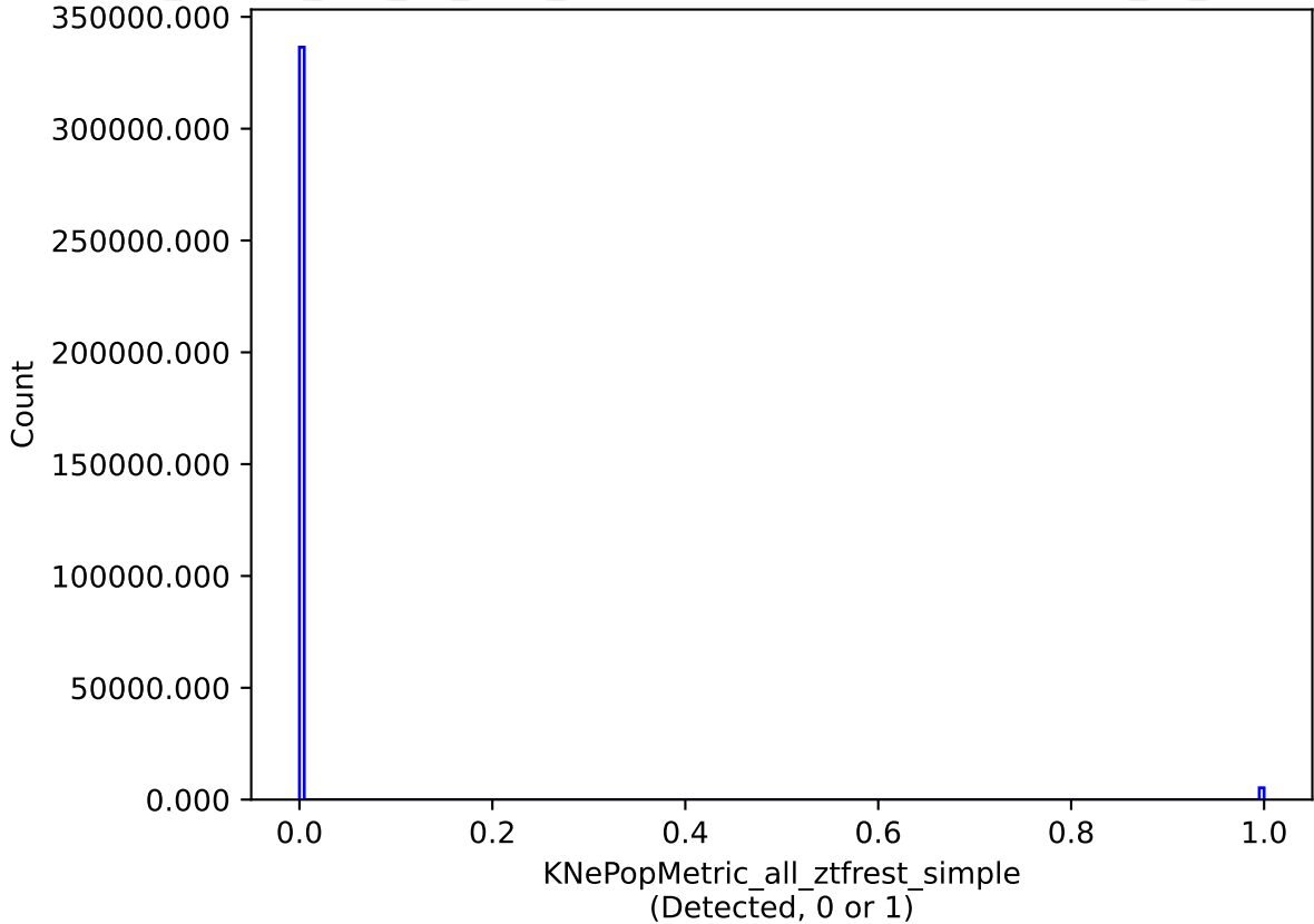
ddf_loaded_half_fl4_v3.4_10yrs all models: KNePopMetric_all_ztfrest_simple
