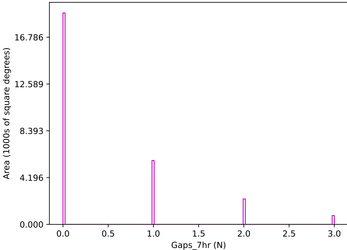
ddf_loaded_half_fl4_v3.4_10yrs z band: Gaps_7hr
