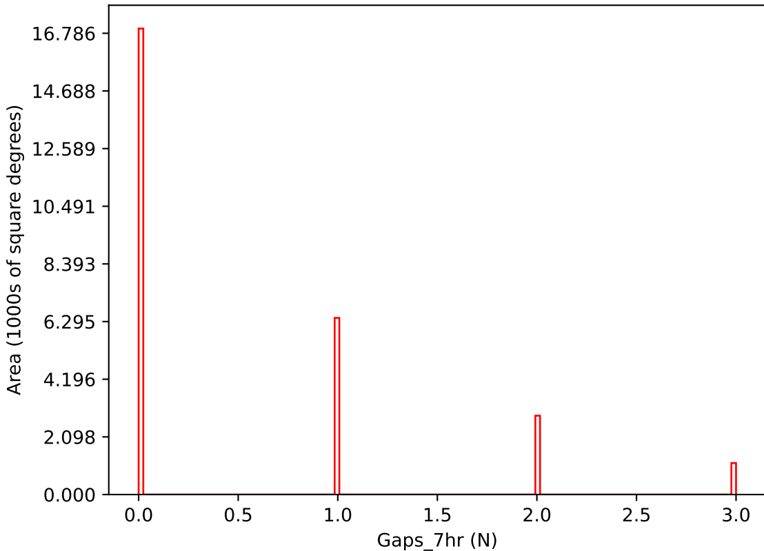
ddf_loaded_half_fl4_v3.4_10yrs i band: Gaps_7hr
