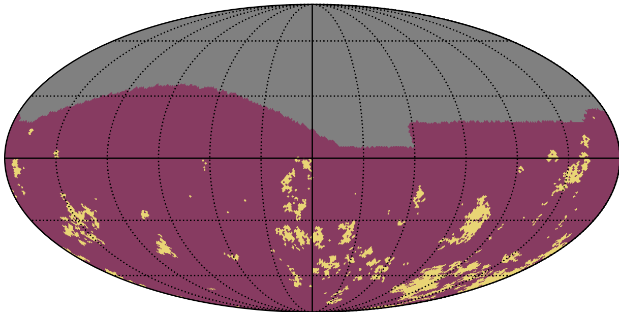
ddf_loaded_half_fl4_v3.4_10yrs g band: Gaps_7hr
