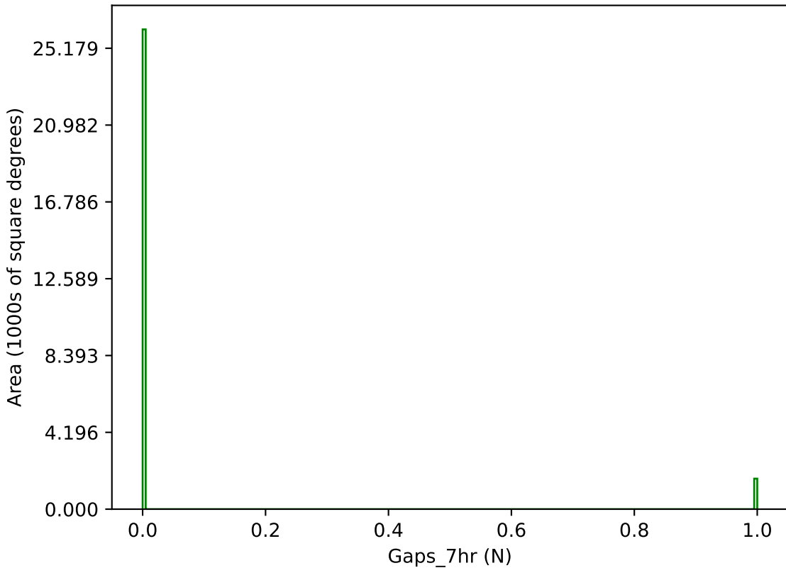
ddf_loaded_half_fl4_v3.4_10yrs g band: Gaps_7hr
