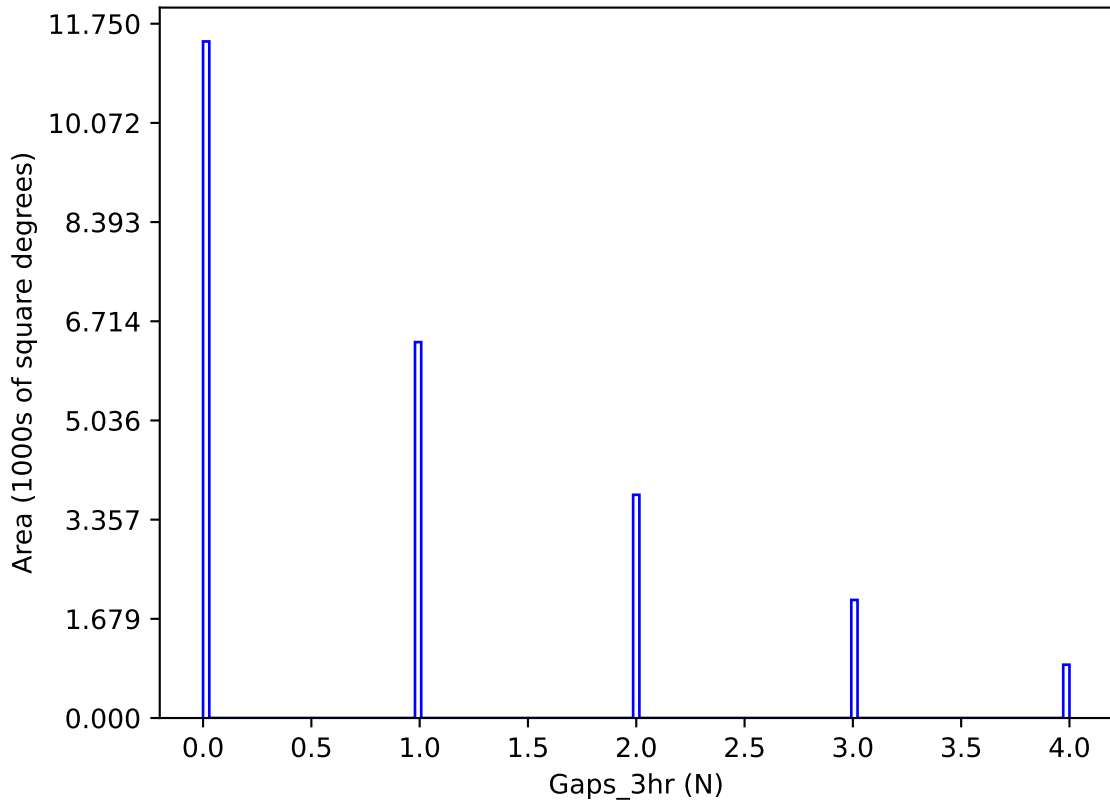
ddf_loaded_half_f14_v3.4_10yrs y band: Gaps_3hr
