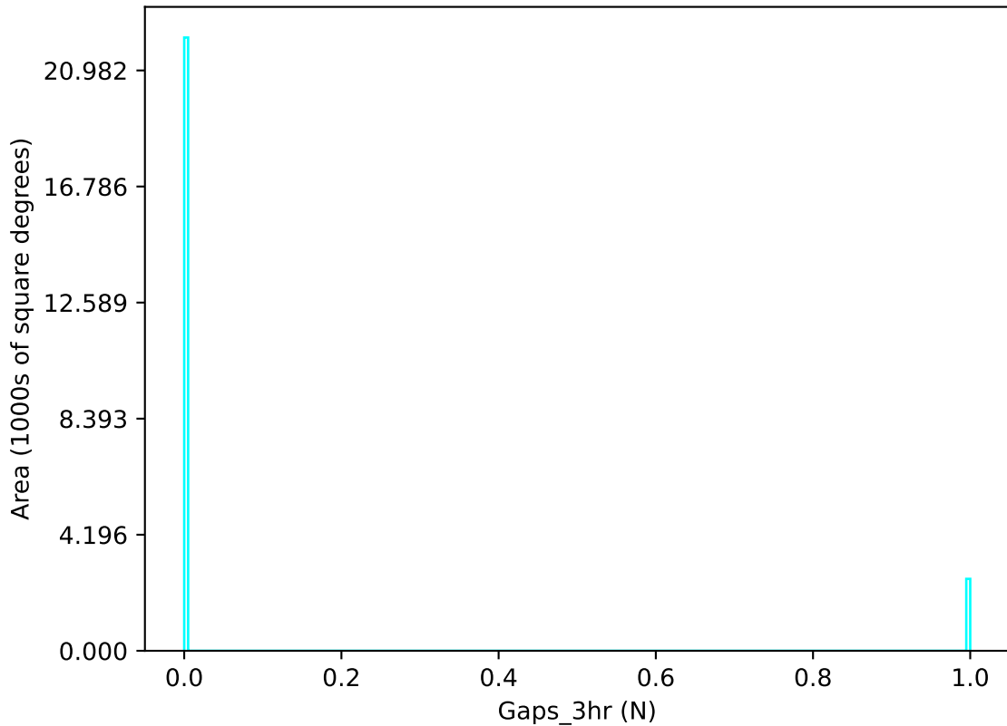
ddf_loaded_half_fl4_v3.4_10yrs u band: Gaps_3hr
