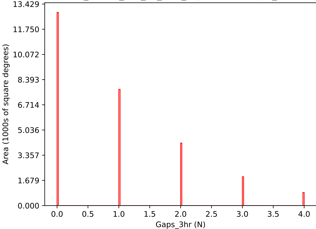
ddf_loaded_half_fl4_v3.4_10yrs i band: Gaps_3hr
