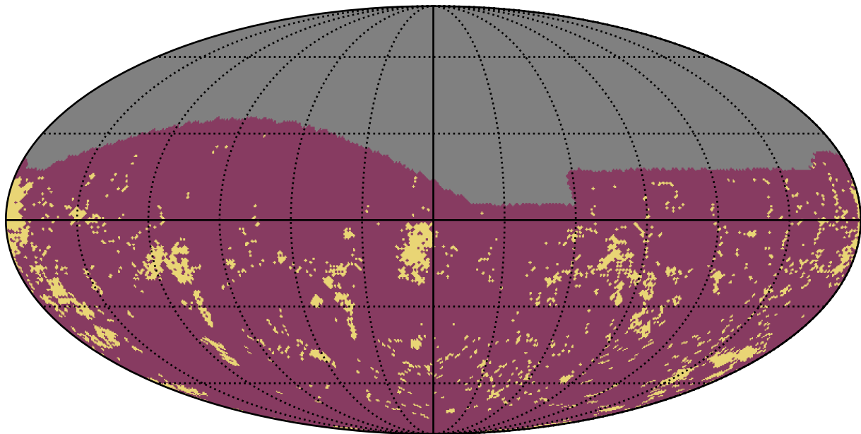
ddf_loaded_half_fl4_v3.4_10yrs g band: Gaps_3hr
