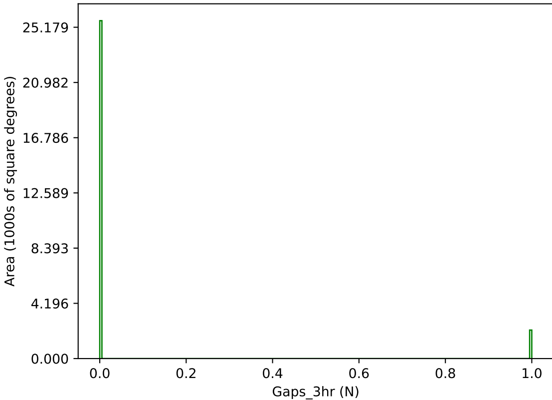
ddf_loaded_half_fl4_v3.4_10yrs g band: Gaps_3hr
