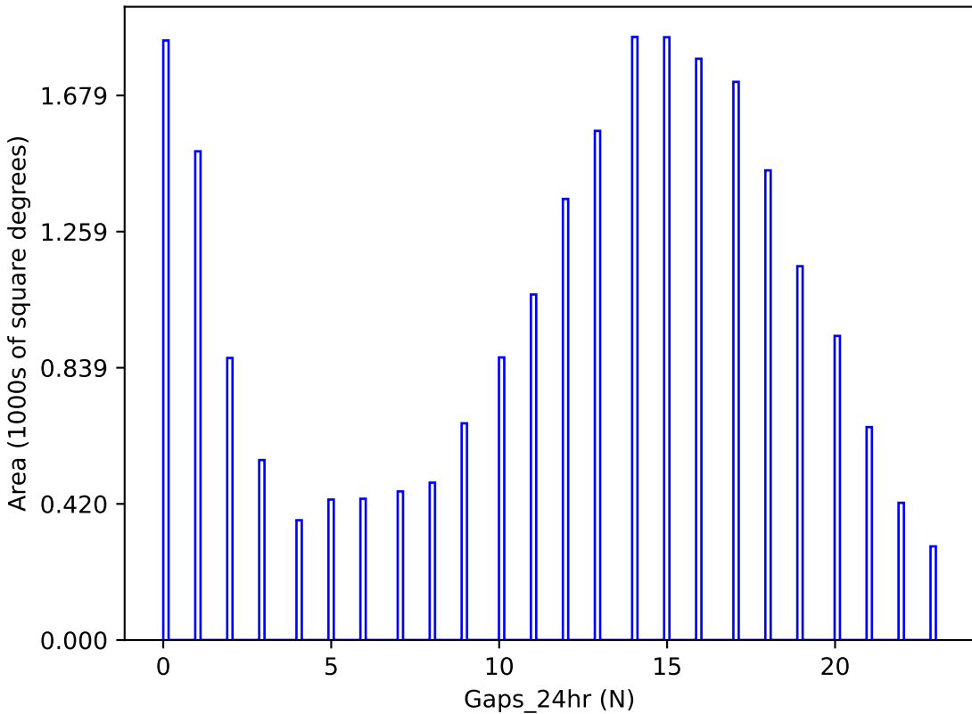
ddf_loaded_half_fl4_v3.4_10yrs y band: Gaps_24hr
