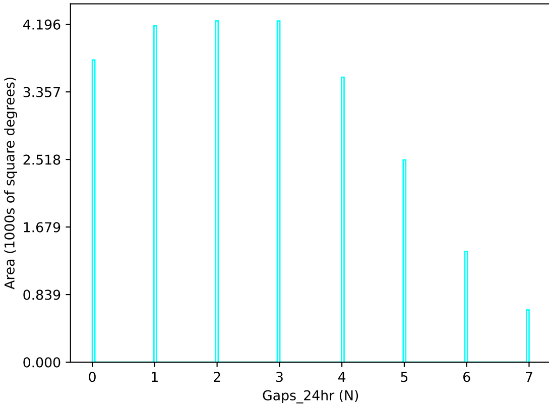
ddf_loaded_half_fl4_v3.4_10yrs u band: Gaps_24hr
