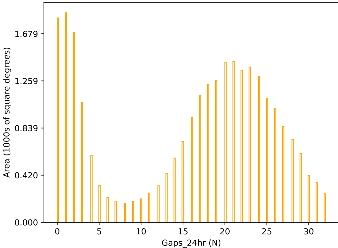
ddf_loaded_half_fl4_v3.4_10yrs r band: Gaps_24hr
