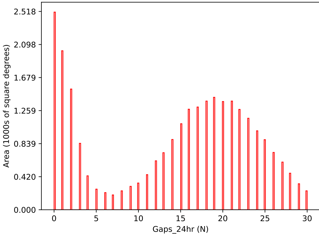
ddf_loaded_half_fl4_v3.4_10yrs i band: Gaps_24hr
