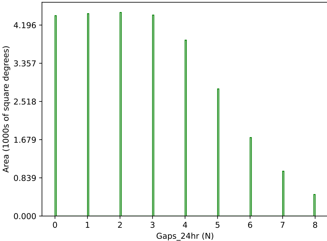
ddf_loaded_half_fl4_v3.4_10yrs g band: Gaps_24hr
