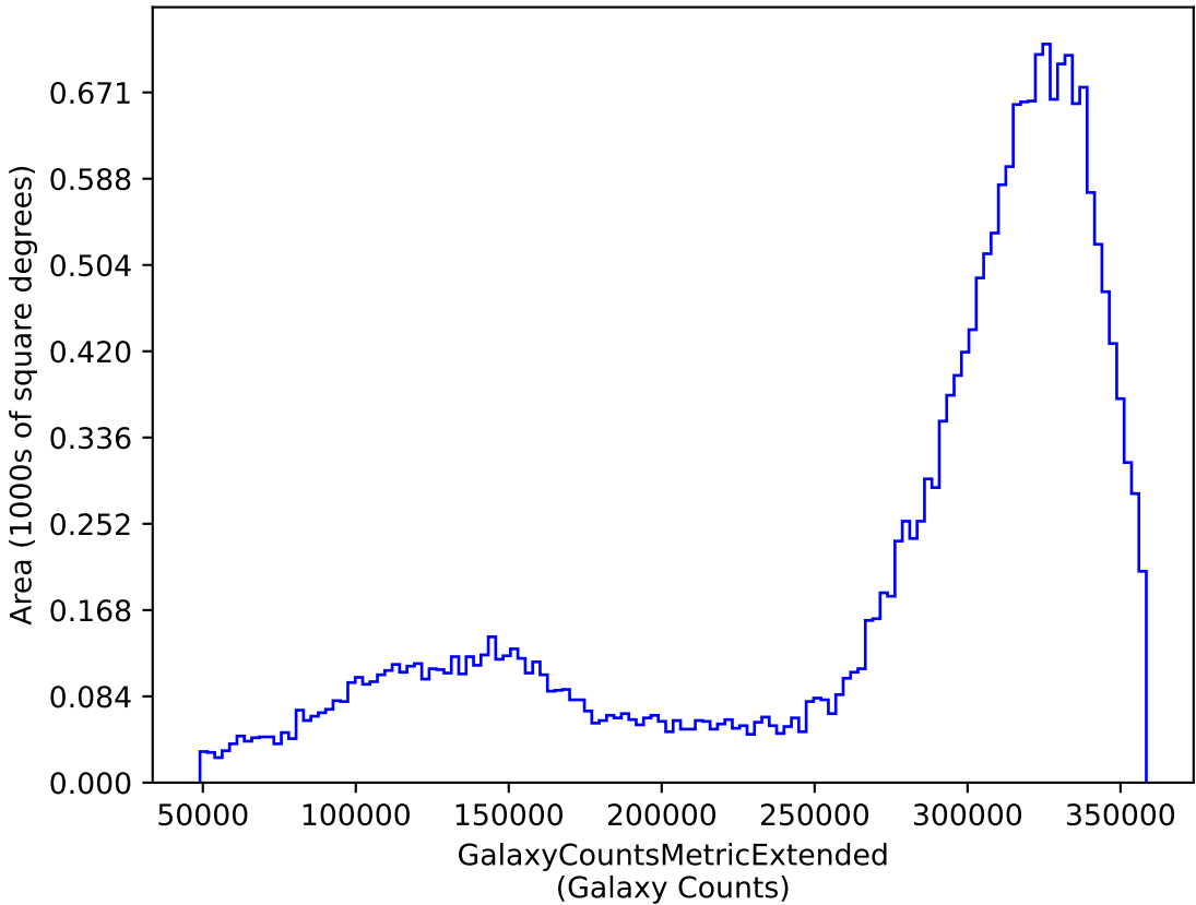
ddf_loaded_half_fl4_v3.4_10yrs y: GalaxyCountsMetricExtended
