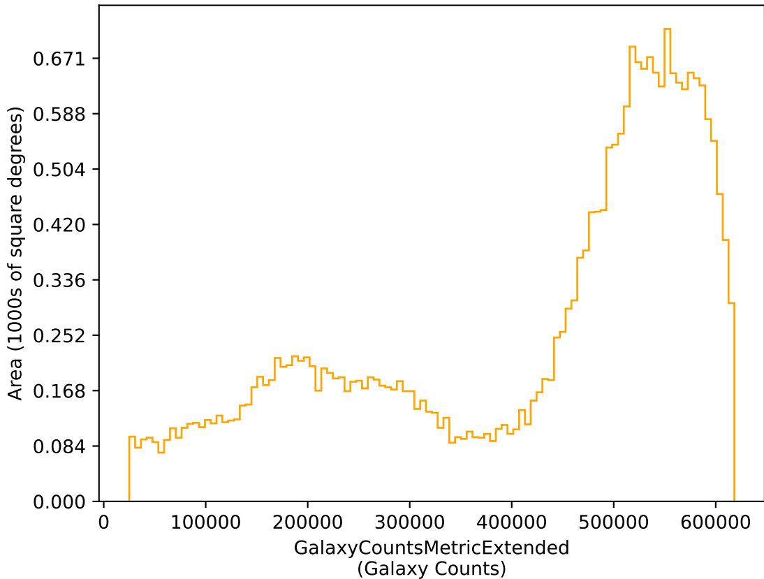
ddf_loaded_half_fl4_v3.4_10yrs r: GalaxyCountsMetricExtended
