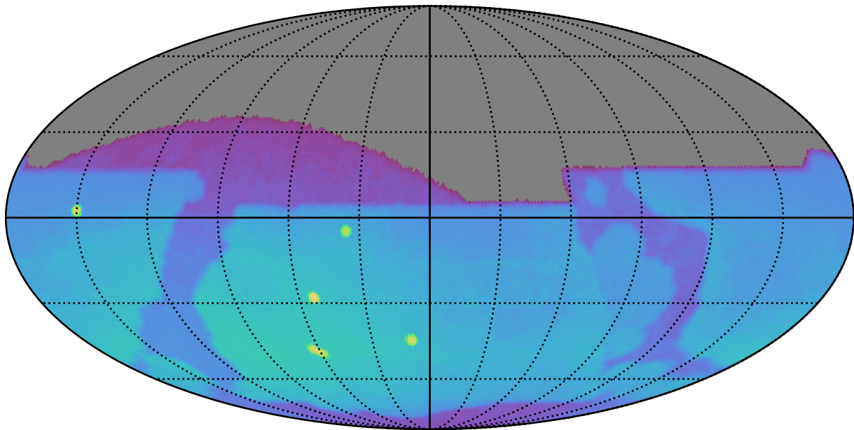
ddf_loaded_half_fl4_v3.4_10yrs : Brown Dwarf, L7
