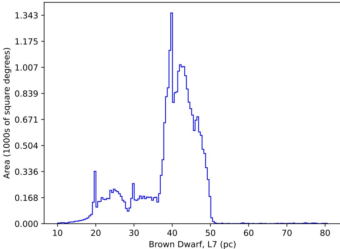
ddf_loaded_half_fl4_v3.4_10yrs : Brown Dwarf, L7
