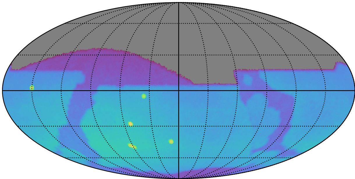
ddf_loaded_half_fl4_v3.4_10yrs : Brown Dwarf, L4
