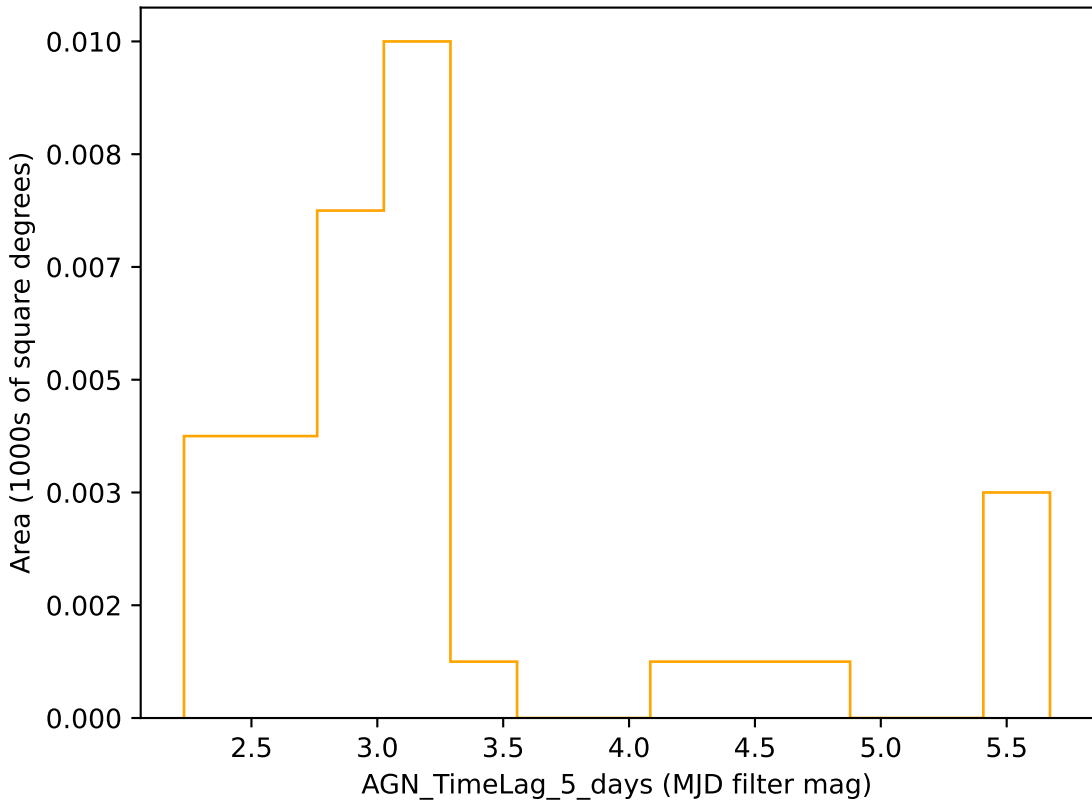
ddf_loaded_half_fl4_v3.4_10yrs r band: AGN_TimeLag_5_days
