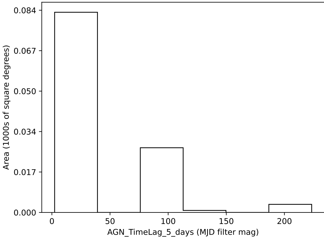
ddf_loaded_half_fl4_v3.4_10yrs all bands: AGN_TimeLag_5_days
