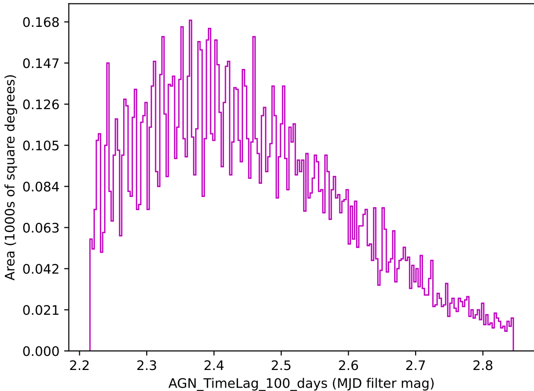
ddf_loaded_half_fl4_v3.4_10yrs z band: AGN_TimeLag_100_days
