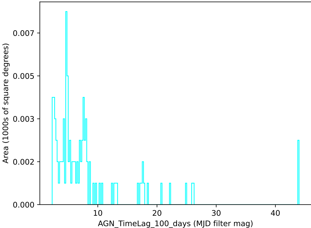
ddf_loaded_half_fl4_v3.4_10yrs u band: AGN_TimeLag_100_days
