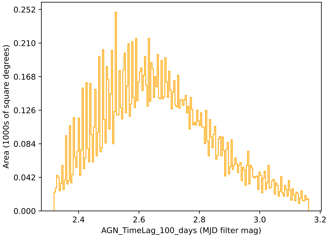
ddf_loaded_half_fl4_v3.4_10yrs r band: AGN_TimeLag_100_days
