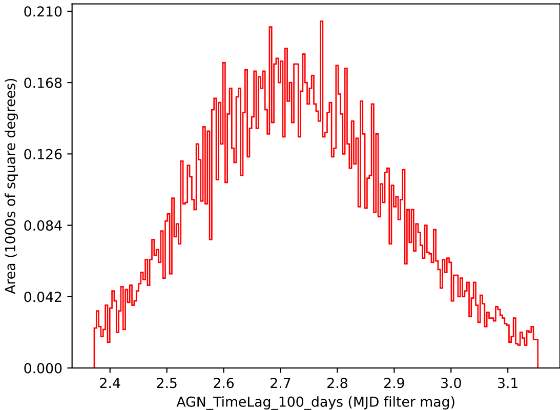
ddf_loaded_half_fl4_v3.4_10yrs i band: AGN_TimeLag_100_days
