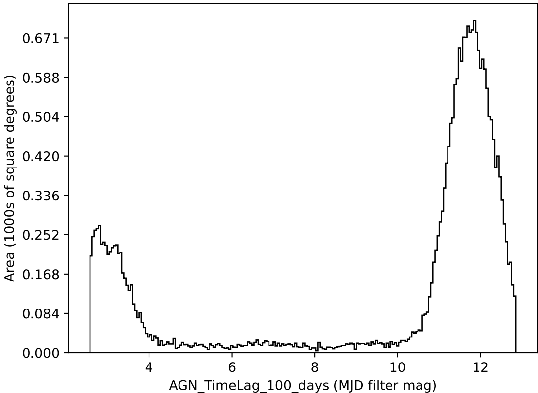
ddf_loaded_half_fl4_v3.4_10yrs all bands: AGN_TimeLag_100_days
