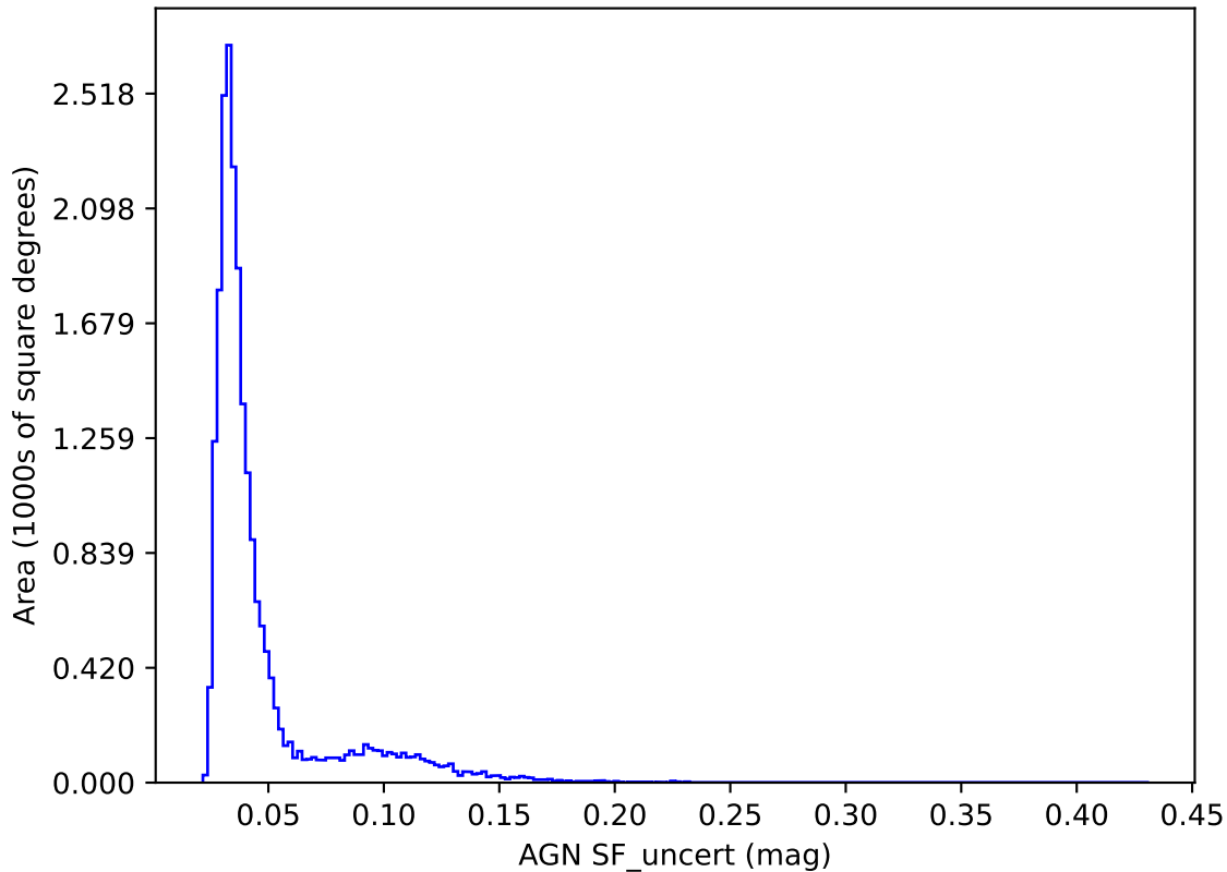
ddf_loaded_half_fl4_v3.4_10yrs y band: AGN SF_uncert
