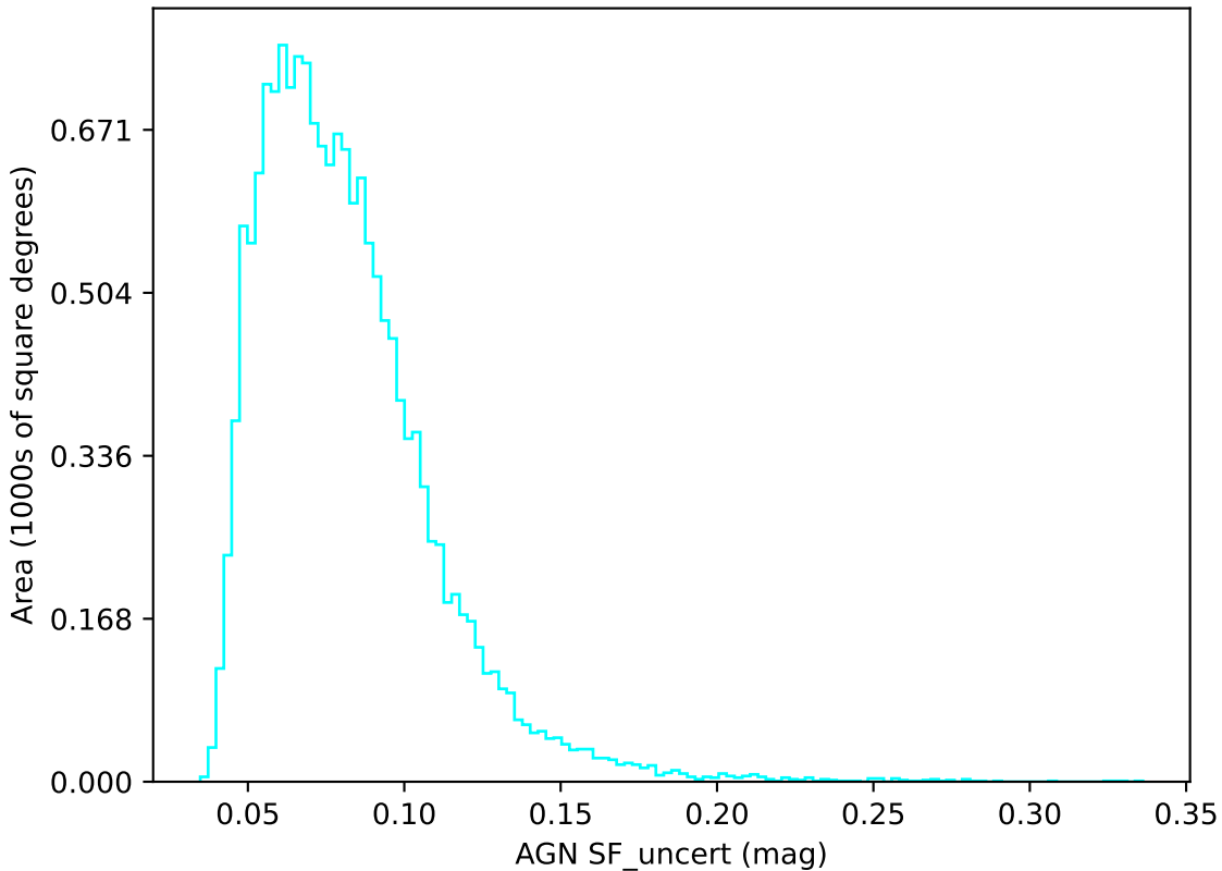
ddf_loaded_half_fl4_v3.4_10yrs u band: AGN SF_uncert
