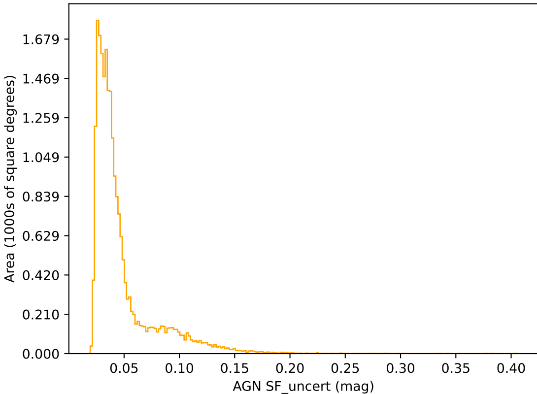
ddf_loaded_half_fl4_v3.4_10yrs r band: AGN SF_uncert
