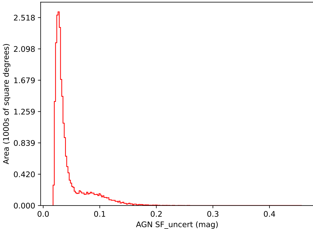
ddf_loaded_half_fl4_v3.4_10yrs i band: AGN SF_uncert
