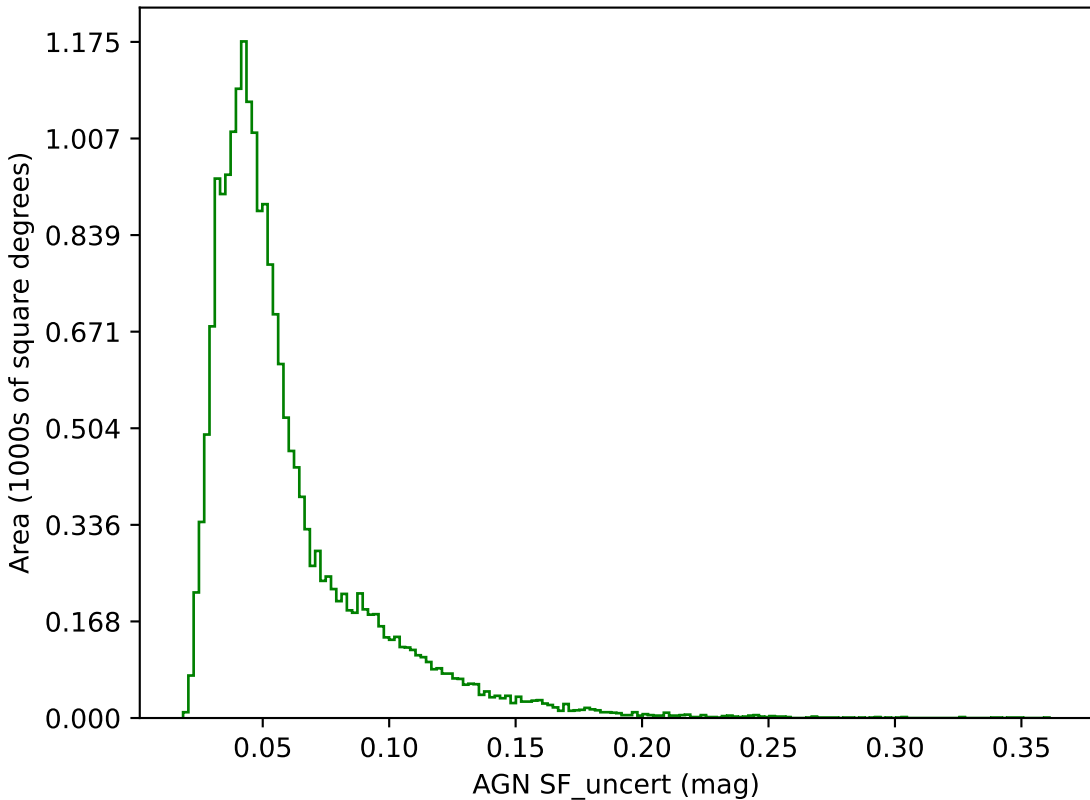
ddf_loaded_half_fl4_v3.4_10yrs g band: AGN SF_uncert
