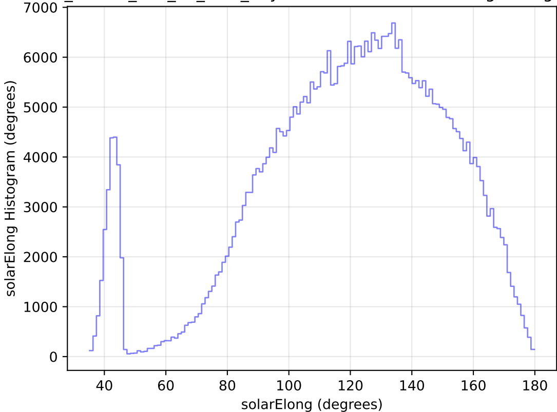
ddf_loaded_half_fl4_v3.4_10yrs WFD z band: solarElong Histogram
