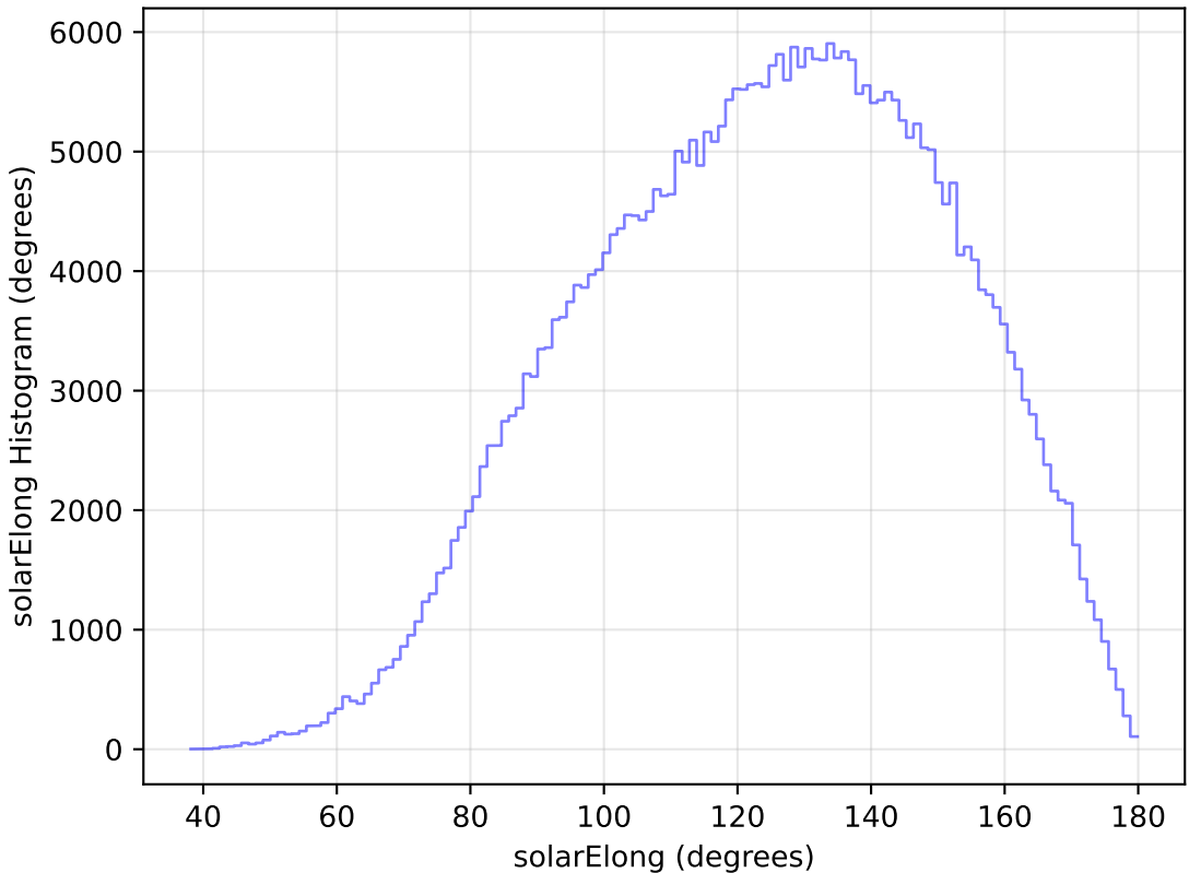
ddf_loaded_half_fl4_v3.4_10yrs WFD y band: solarElong Histogram
