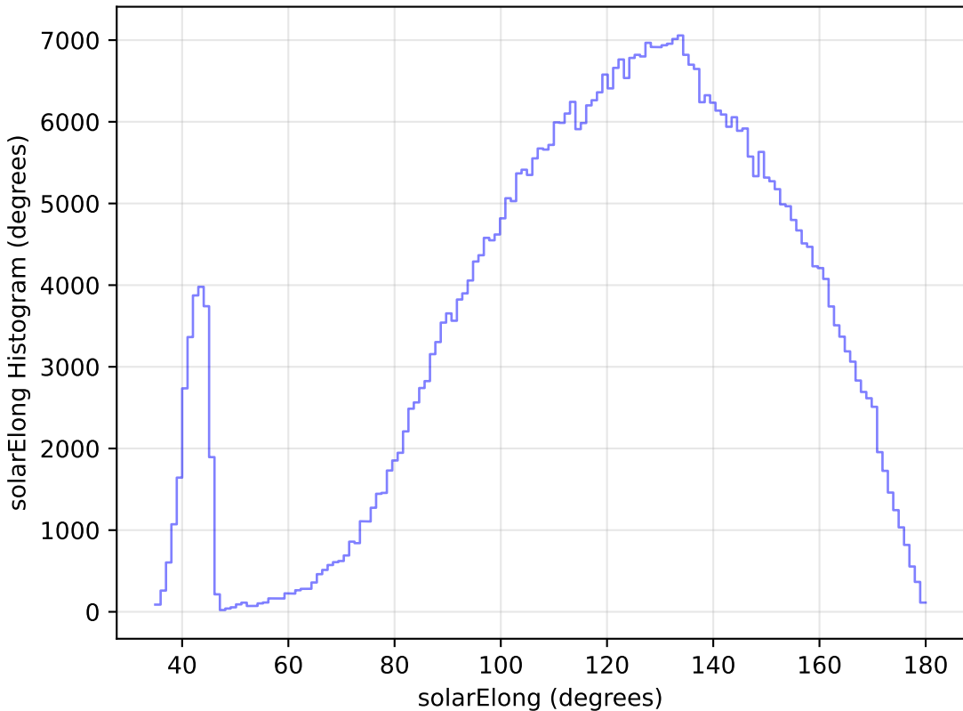
ddf_loaded_half_fl4_v3.4_10yrs WFD i band: solarElong Histogram
