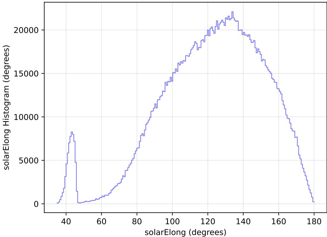
ddf_loaded_half_fl4_v3.4_10yrs WFD all bands: solarElong Histogram
