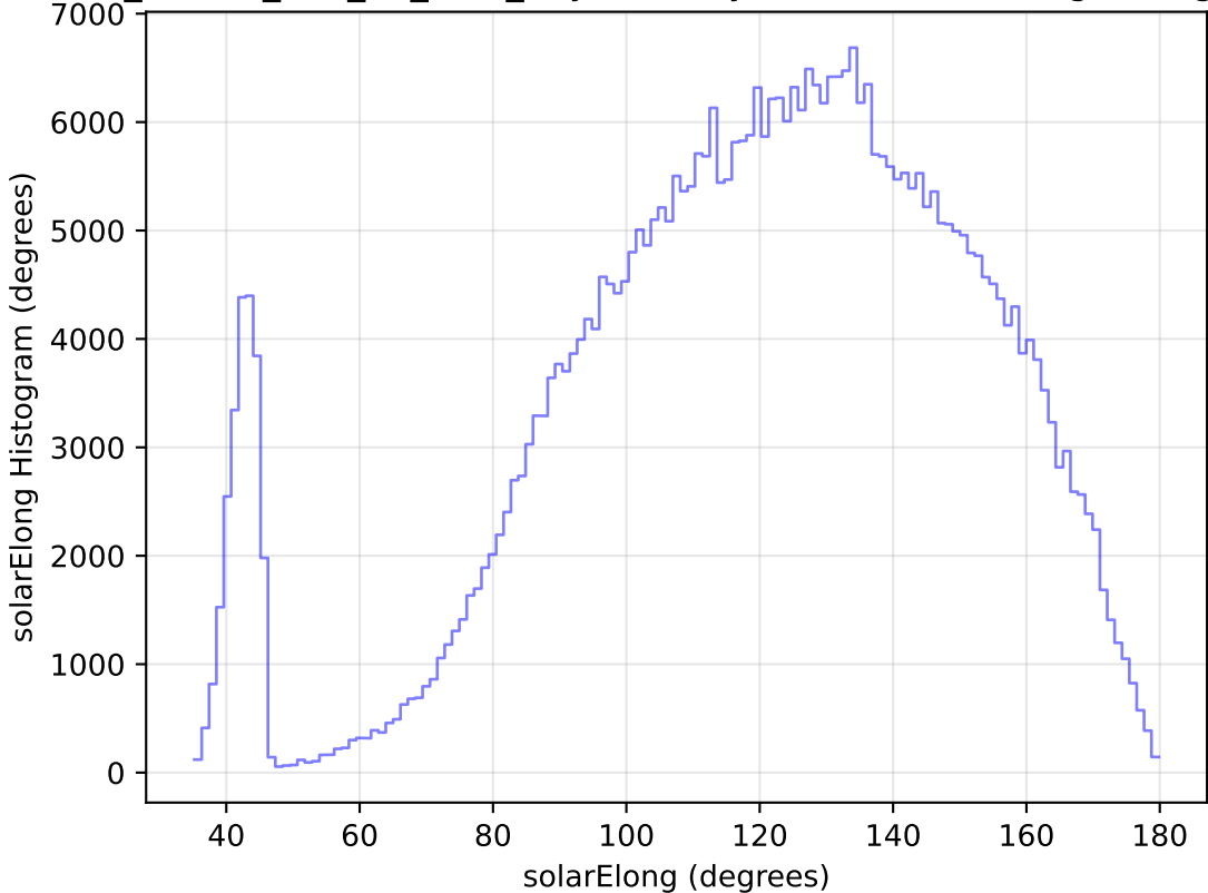
ddf_loaded_half_fl4_v3.4_10yrs All sky z band: solarElong Histogram
