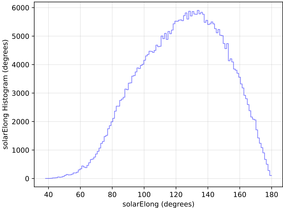
ddf_loaded_half_fl4_v3.4_10yrs All sky y band: solarElong Histogram
